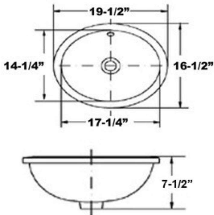
I/D 17-1/4"W x 14-1/4"D x 6"Depth
